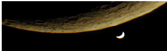
Lunar occultation of Venus April 22nd, 2009
